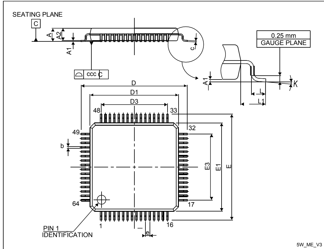
Figure 44. LQFP64 package outline
