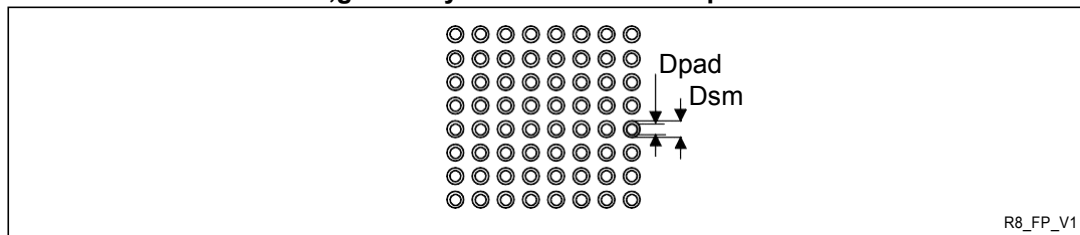
Figure 41. TFBGA64 – 64-ball, 5 x 5 mm, 0.5 mm pitch, thin profile fine pitch ball grid array recommended footprint
