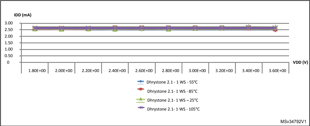
Figure 13. I_{DD} vs V_{DD} , at T_A = 25/55/85/105\text{ }^{\circ}\text{C} , Run mode, code running from Flash memory, Range 2, HSI16, 1WS
