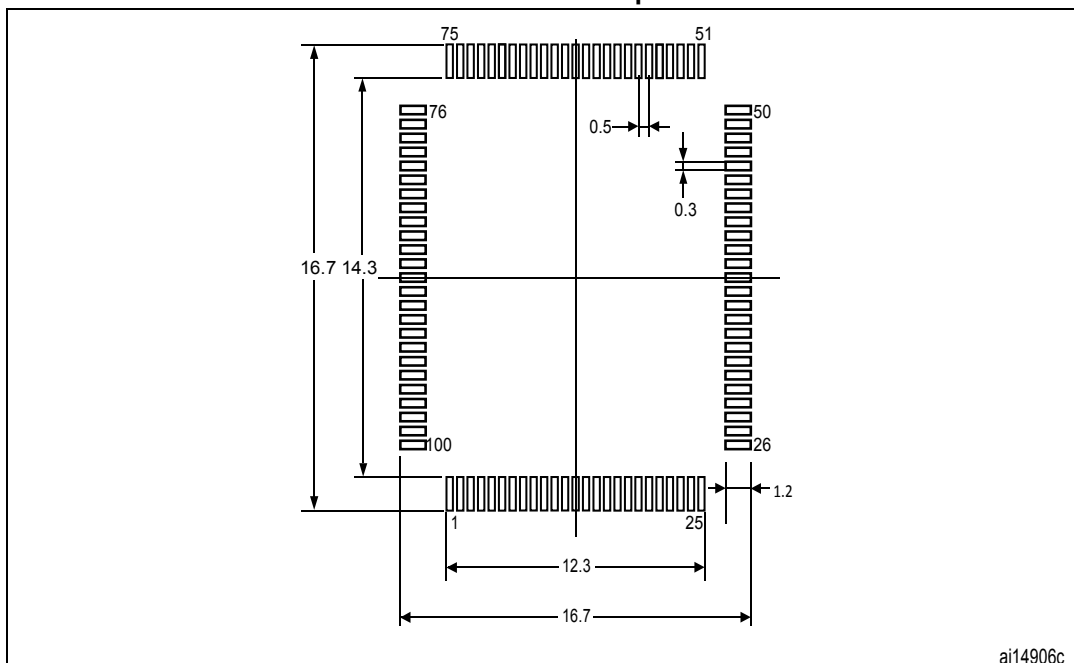
Figure 40. LQFP100 - 100-pin, 14 x 14 mm low-profile quad flat package recommended footprint
