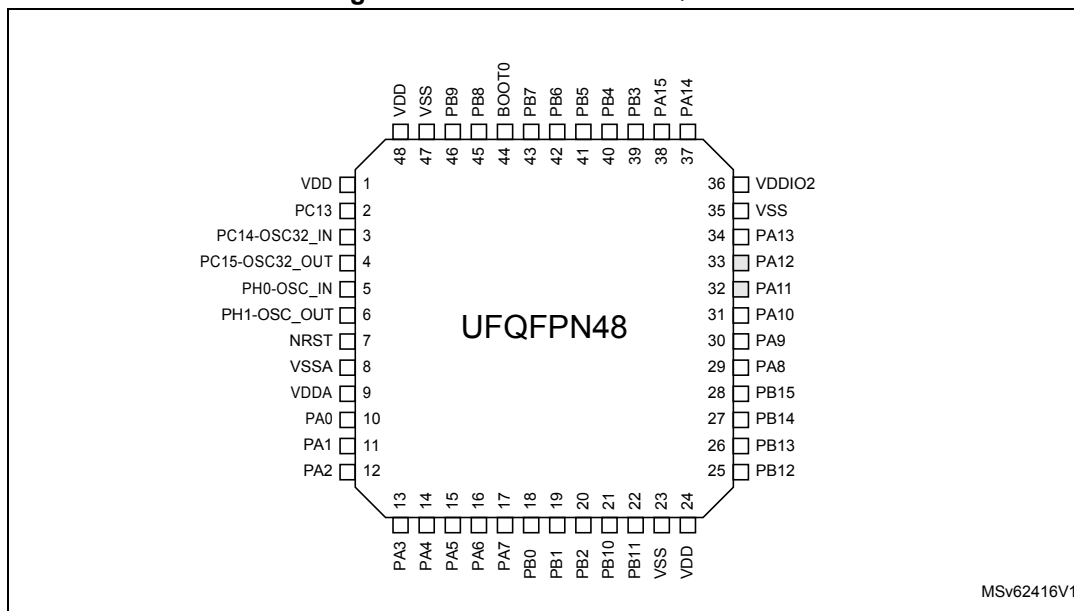
Figure 9. STM32L071xx UFQFPN48
