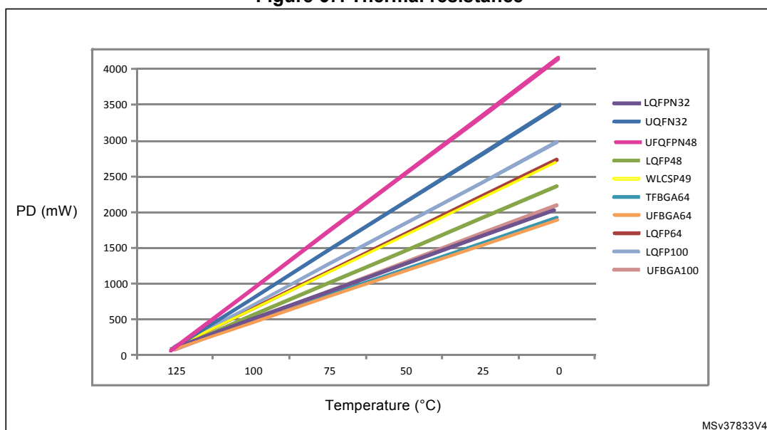
Figure 67. Thermal resistance
