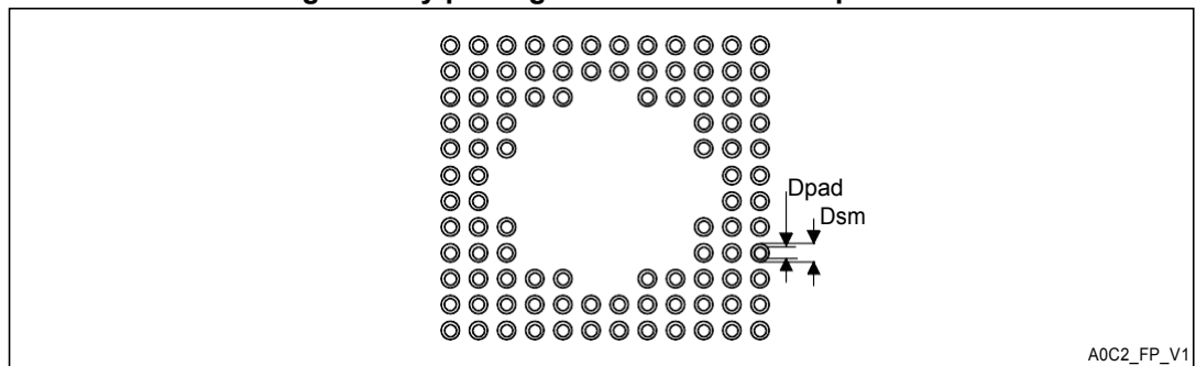
Figure 43. UFBGA100 - 100-pin, 7 x 7 mm, 0.50 mm pitch, ultra fine pitch ball grid array package recommended footprint
