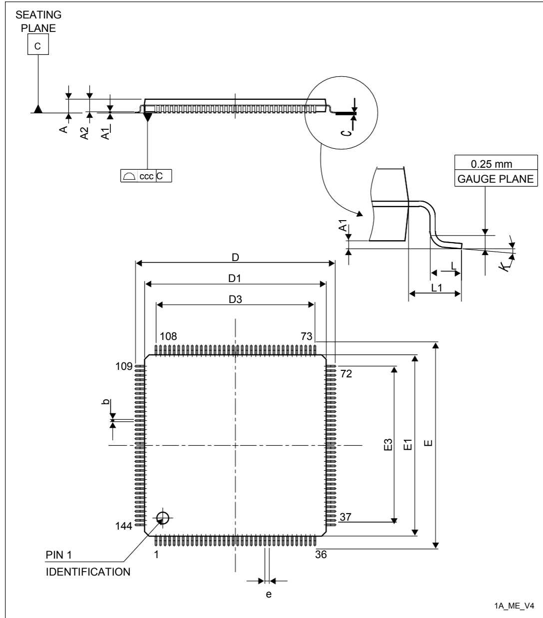
Figure 84. LQFP144 outline
