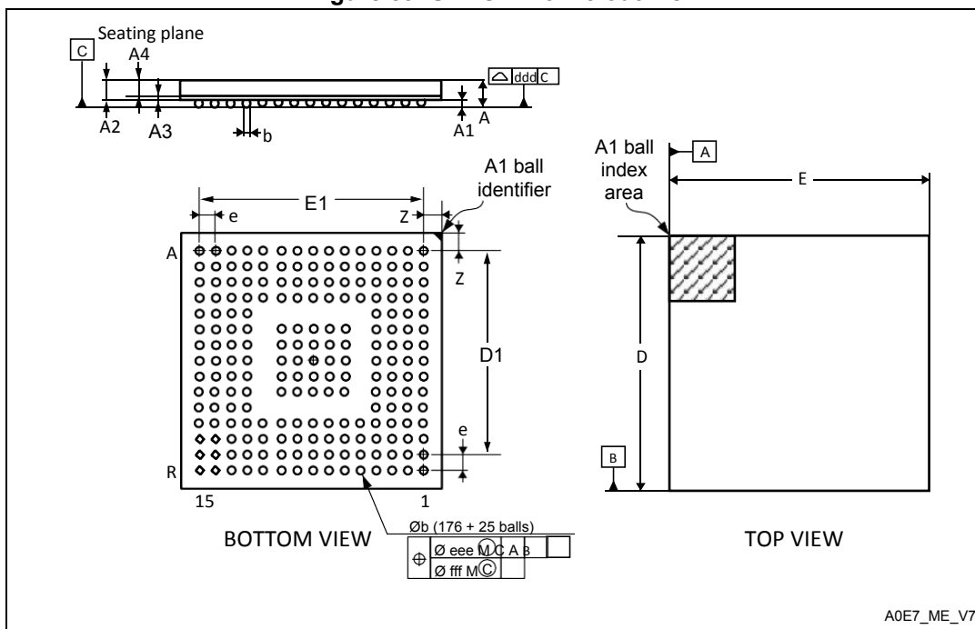
Figure 89. UFBGA176+25 outline
