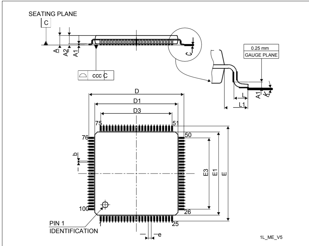
Figure 81. LQFP100 outline
