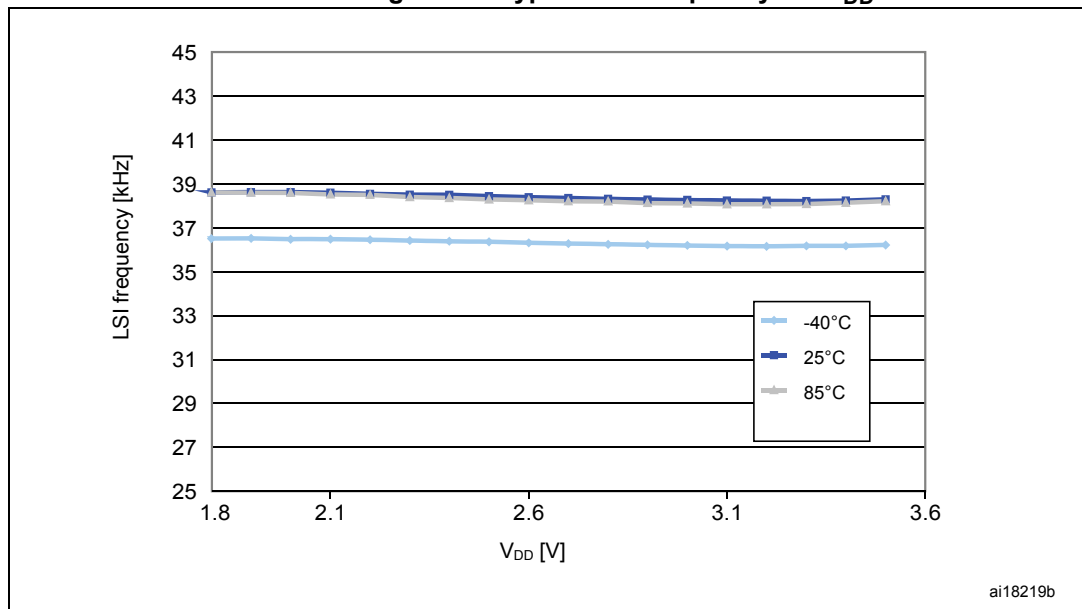
Figure 15. Typical LSI frequency vs. V_{\text{DD}}
