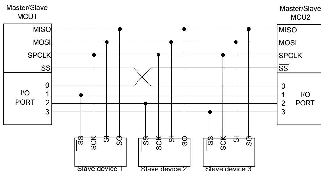
Figure 14.2. SPI Multi-Master, Multi-Slave Interconnection
