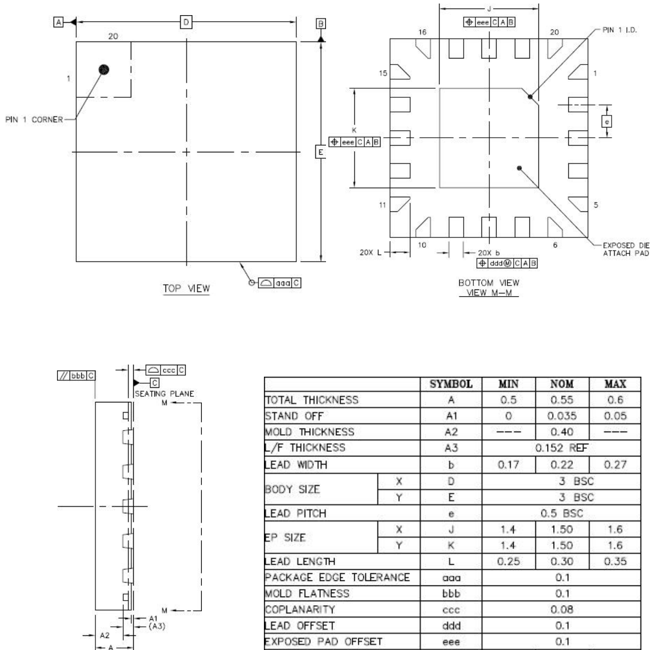
Figure 32.4. QFN-20 Package Dimension of N76E003BQ20
