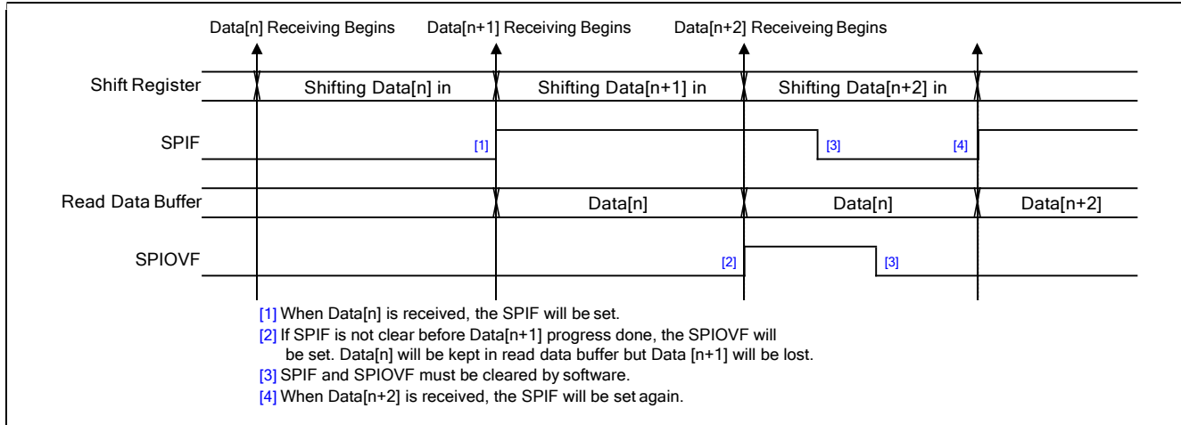
Figure 14.7. SPI Overrun Waveform
