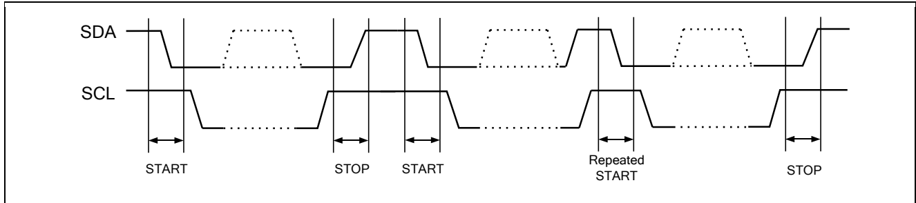
Figure 15.3. START, Repeated START, and STOP Conditions
