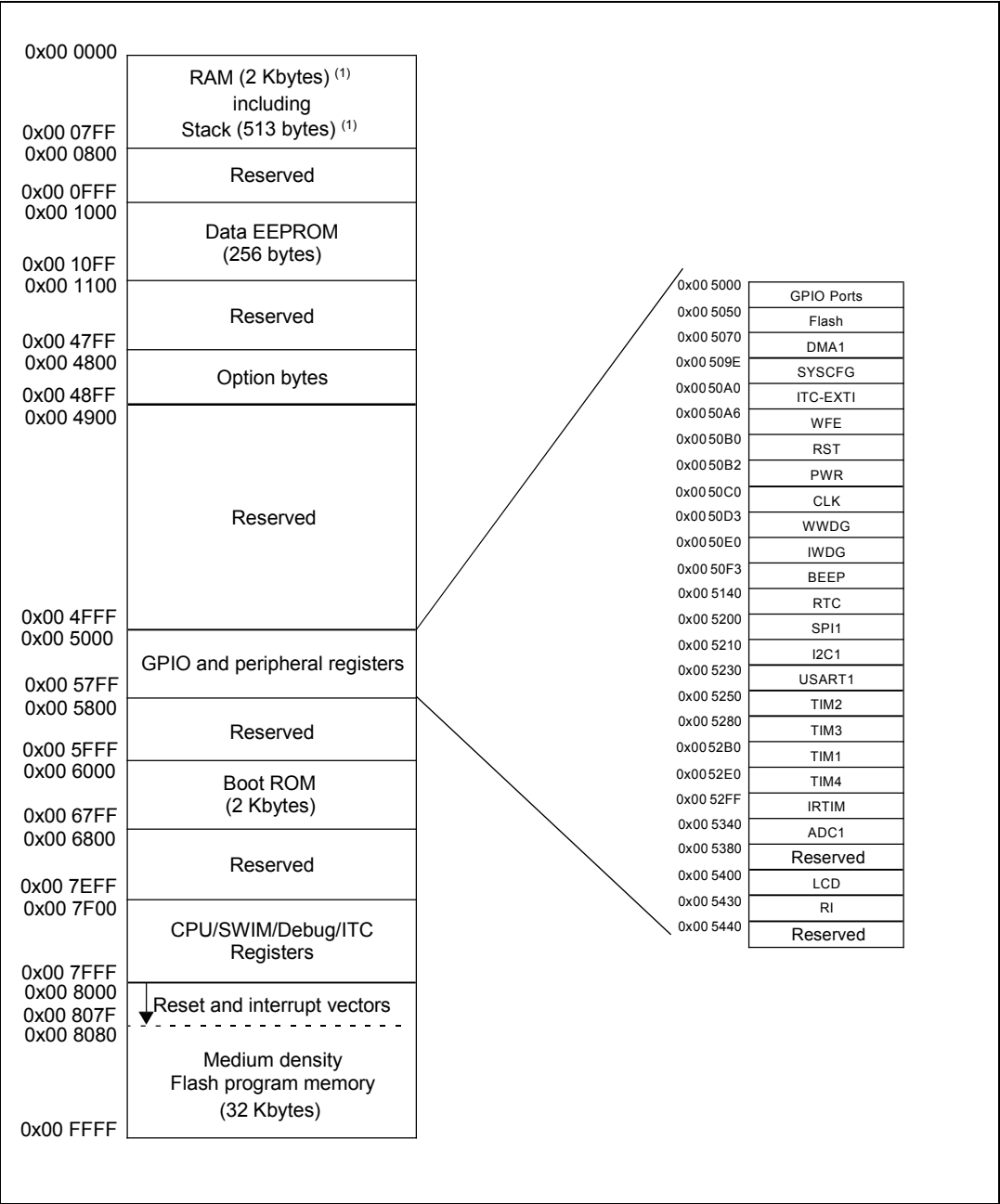
Figure 4. Memory map
