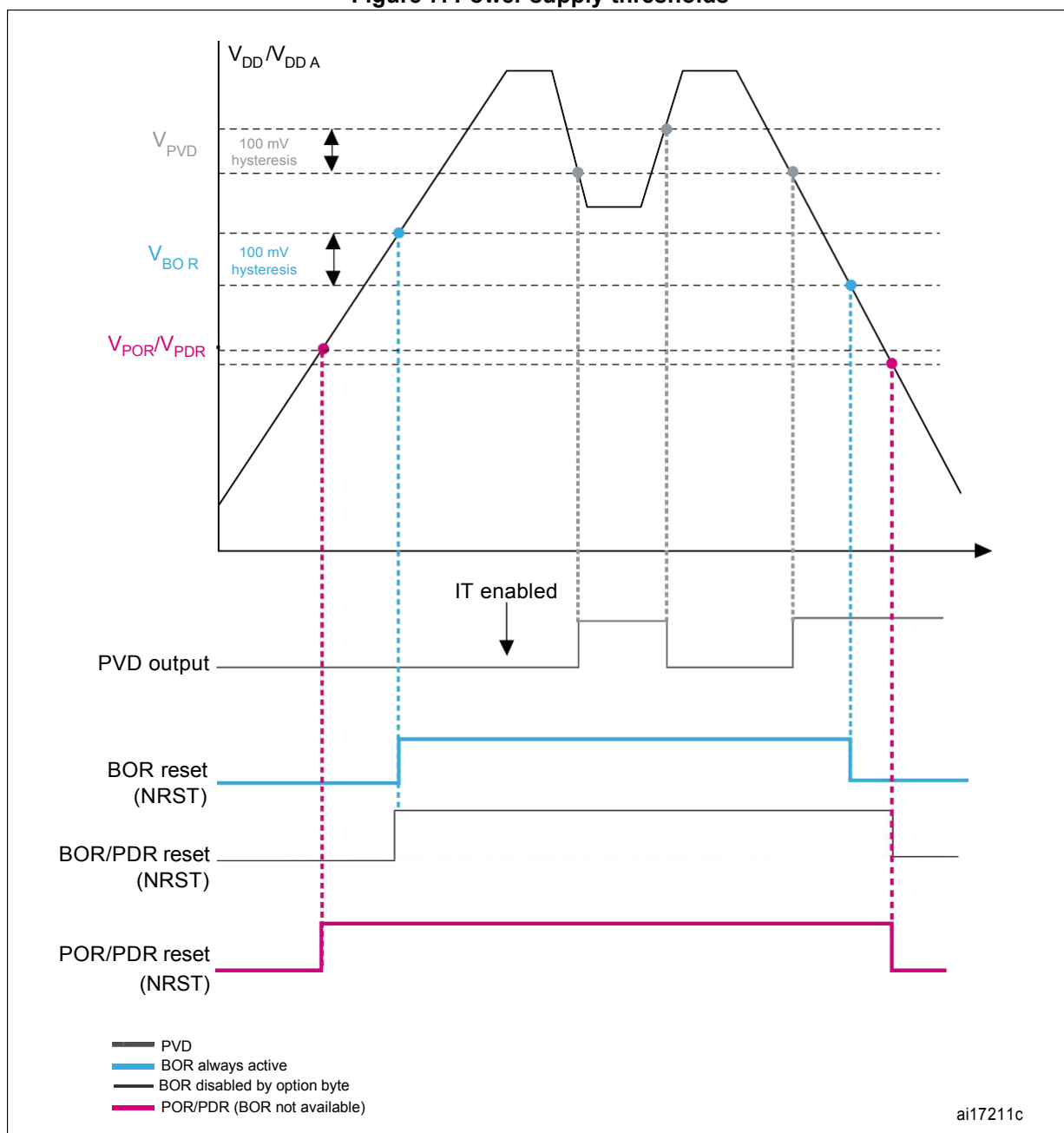
Figure 7. Power supply thresholds
