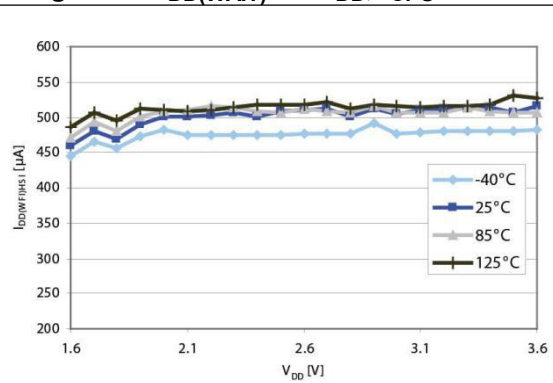
Figure 14. I_{DD(WAIT)} vs. V_{DD} , f_{CPU} = 16 \text{ MHz}
