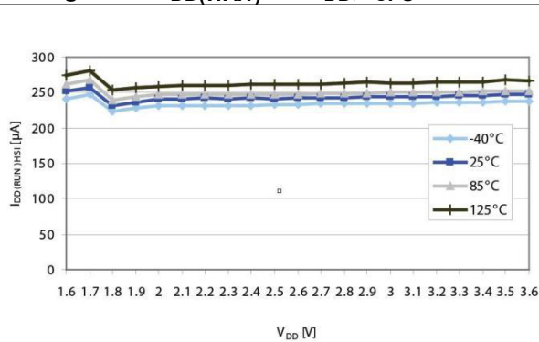
Figure 13. I_{DD(WAIT)} vs. V_{DD} , f_{CPU} = 2 \text{ MHz}
