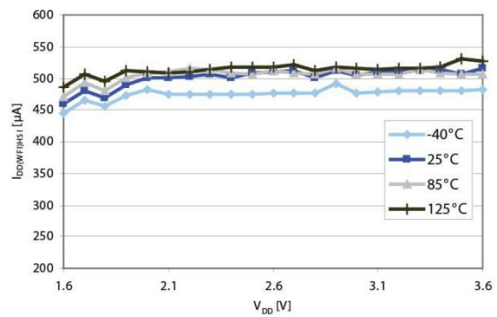
Figure 14. I_{DD(WAIT)} vs. V_{DD} , f_{CPU} = 16 \text{ MHz}
