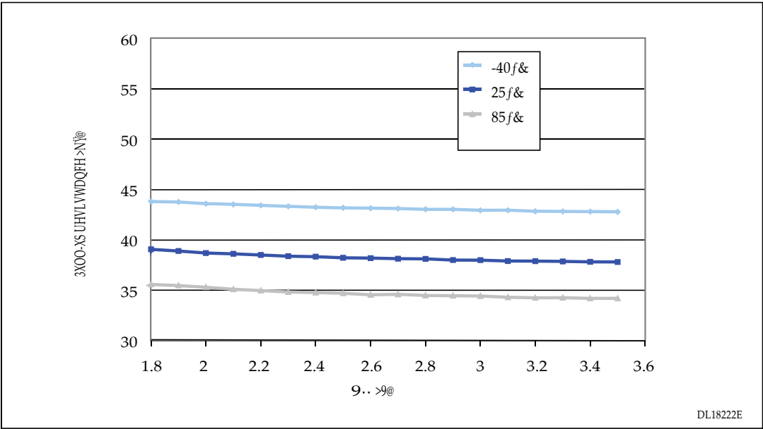
Figure 23. Typical pull-up resistance R_{PU} vs V_{DD} with V_{IN}=V_{SS}
