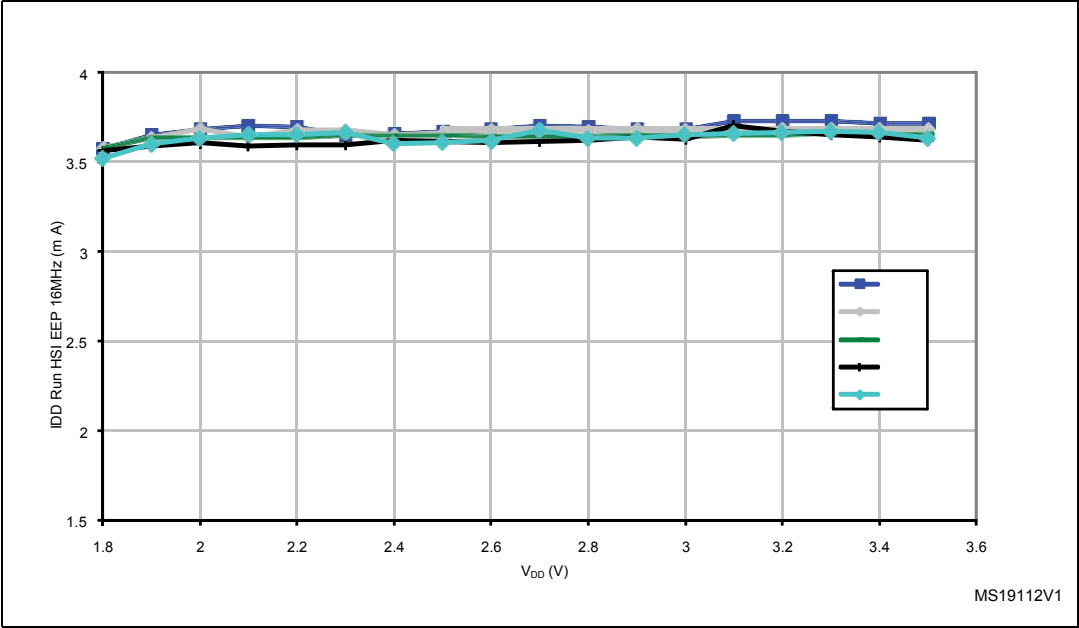
Figure 15. Typical I_{DD(RUN)} from Flash vs. V_{DD} (HSI clock source), f_{CPU}=16\text{ MHz}
