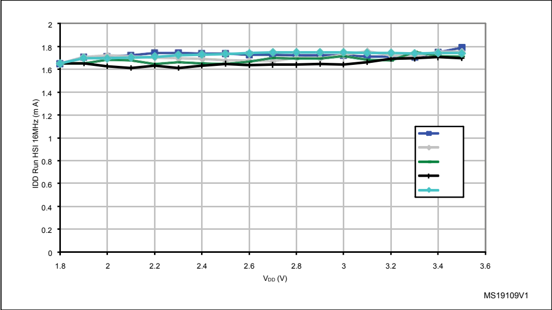
Figure 14. Typical I_{DD(RUN)} from RAM vs. V_{DD} (HSI clock source), f_{CPU}=16\text{ MHz}
