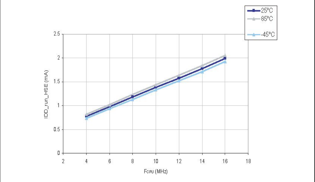
Figure 12. Typ. I_{DD(RUN)} vs f_{CPU} , HSE user external clock, V_{DD} = 5\text{ V}
