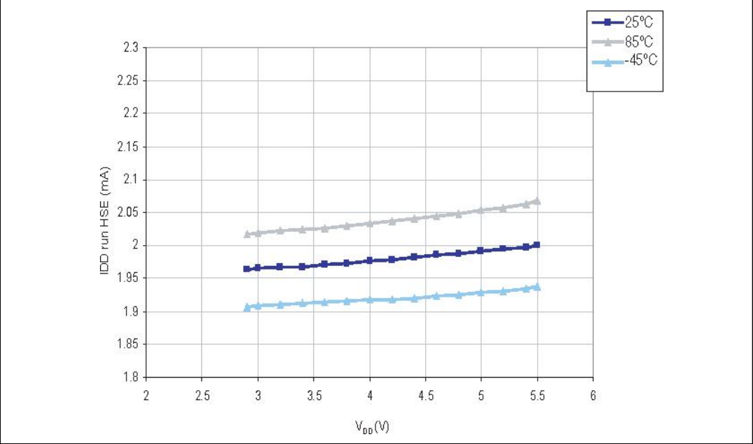
Figure 11. Typ. I_{DD(RUN)} vs V_{DD} , HSE user external clock, f_{CPU} = 16\text{ MHz}
