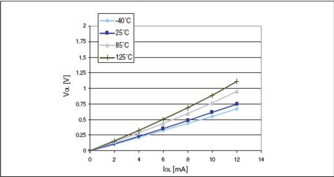
Figure 27. Typ. V_{OL} @ V_{DD} = 3.3\text{ V} (true open drain ports)
