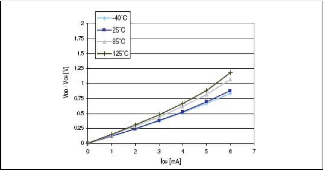
Figure 31. Typ. V_{DD} - V_{OH} @ V_{DD} = 3.3\text{ V} (standard ports)
