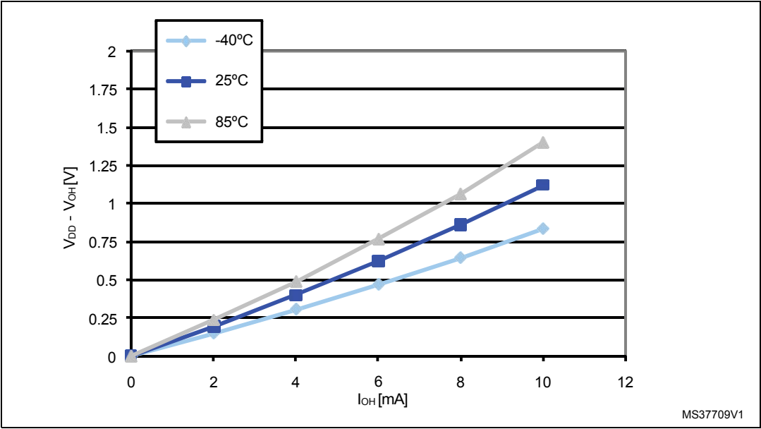
Figure 30. Typ. V_{DD} - V_{OH} @ V_{DD} = 5\text{ V} (standard ports)
