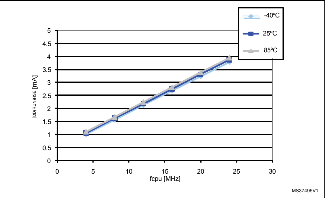
Figure 12. Typ. I_{DD(RUN)} vs f_{CPU} , HSE user external clock, V_{DD} = 5\text{ V}
