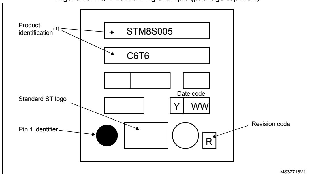
Figure 46. LQFP48 marking example (package top view)
