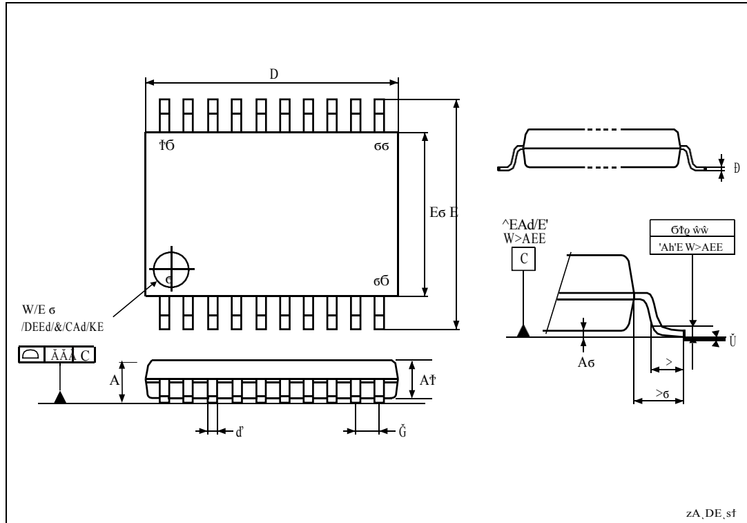
Figure 46.TSSOP20 package outline
