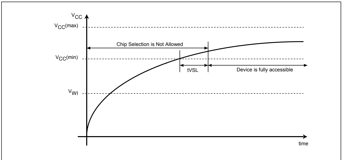
Figure 49. Power-up Timing
