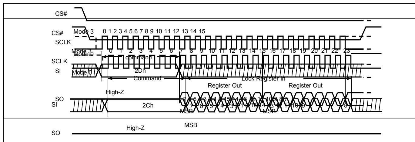
Figure 70. Write Lock Register (WRLR) Sequence
