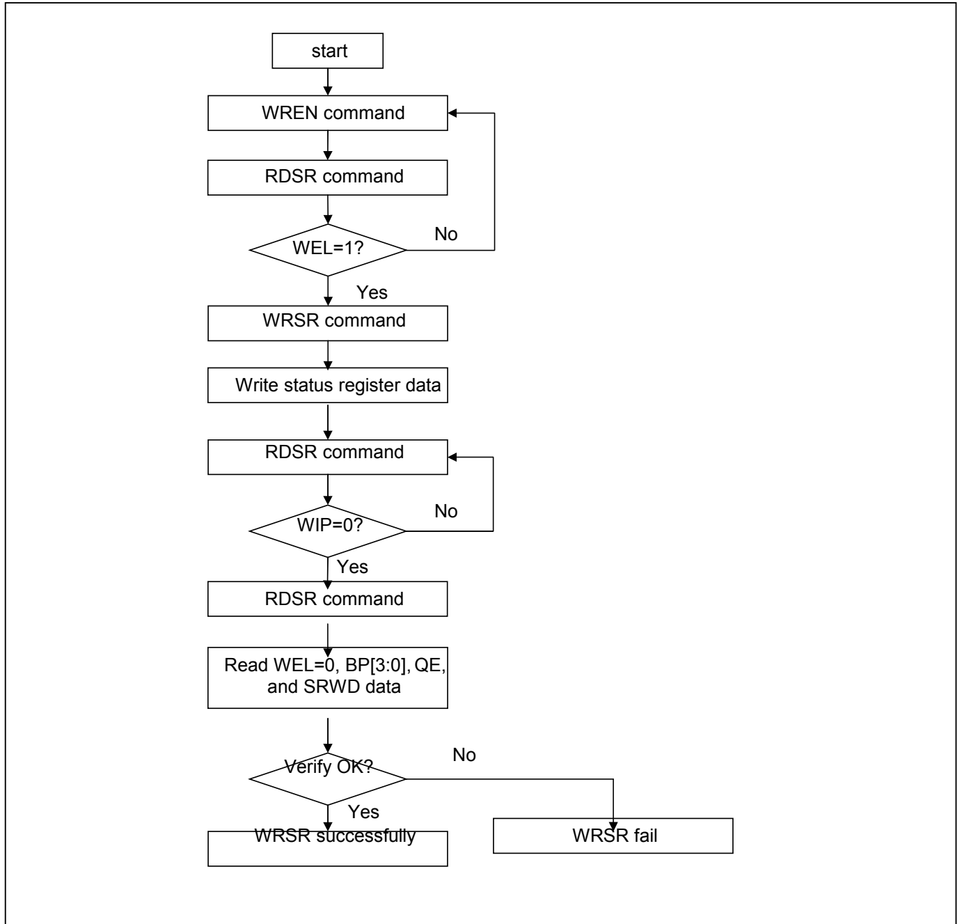
Figure 27. WRSR flow
