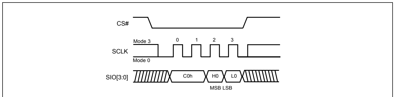
Figure 33. QPI Mode
