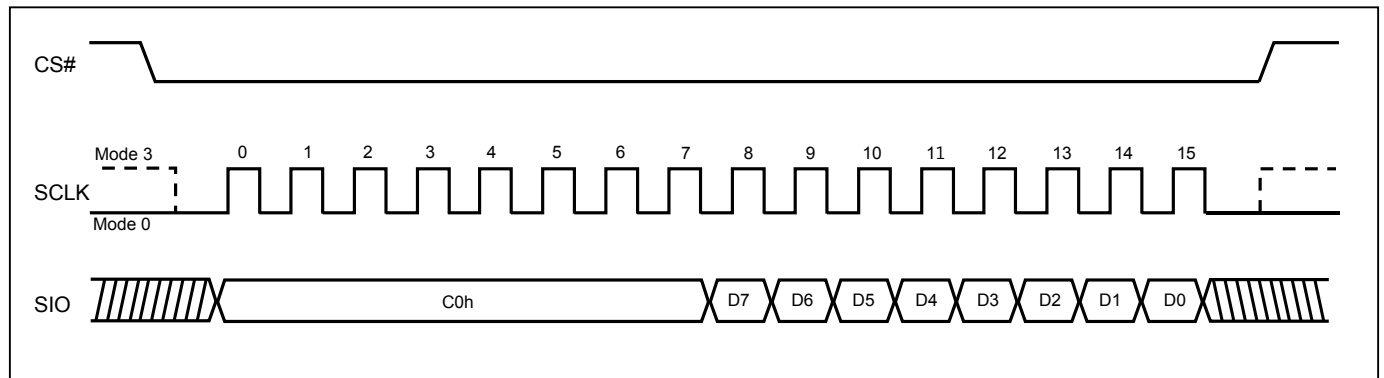
Figure 32. SPI Mode
