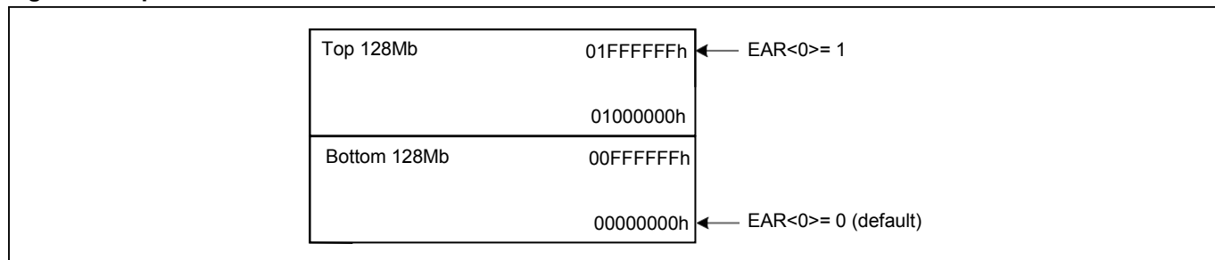
Figure 6. Top and Bottom 128M bits
