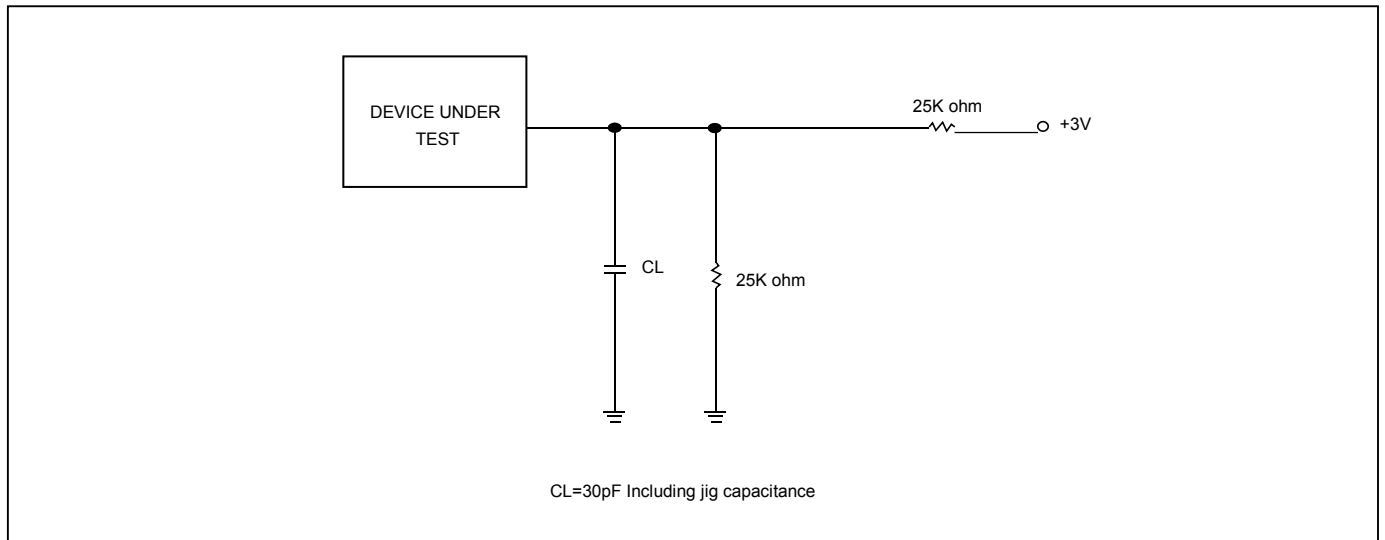
Figure 93. OUTPUT LOADING
