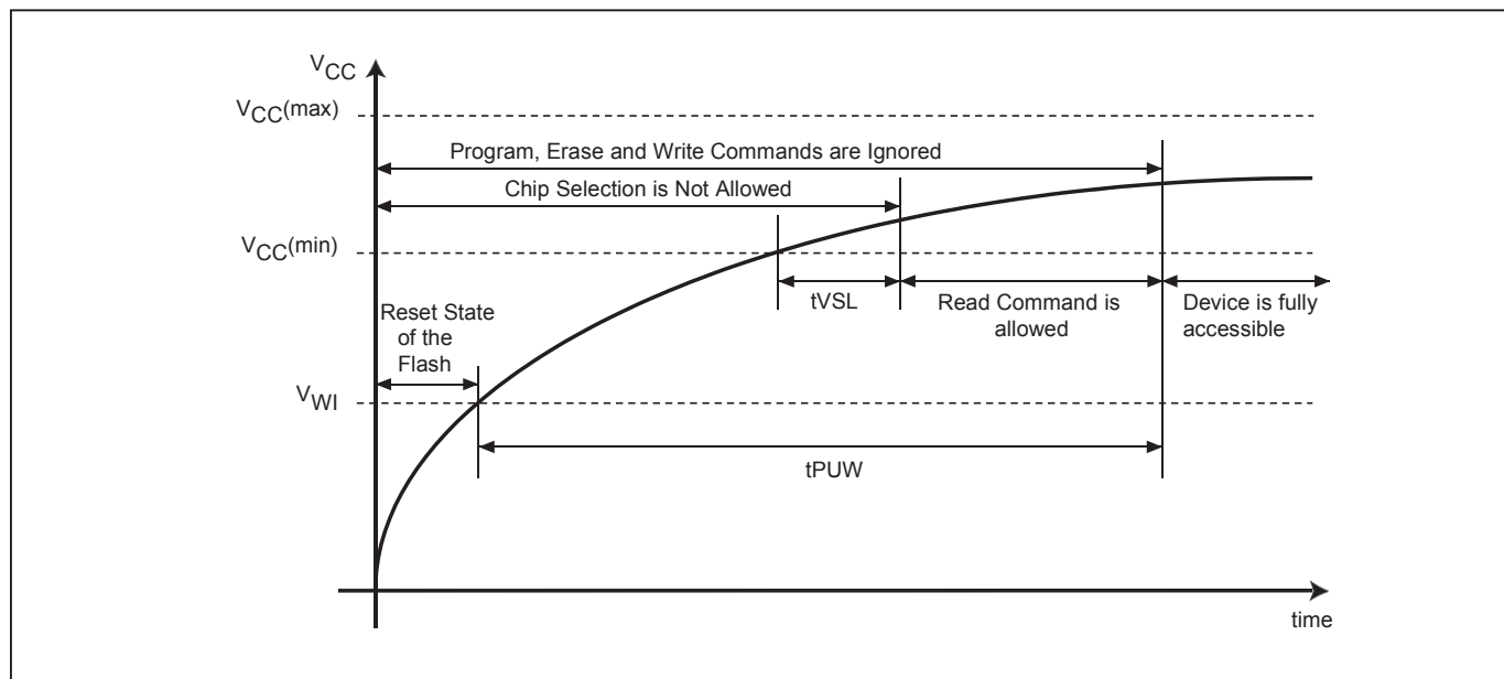
Figure 36. Power-up Timing
