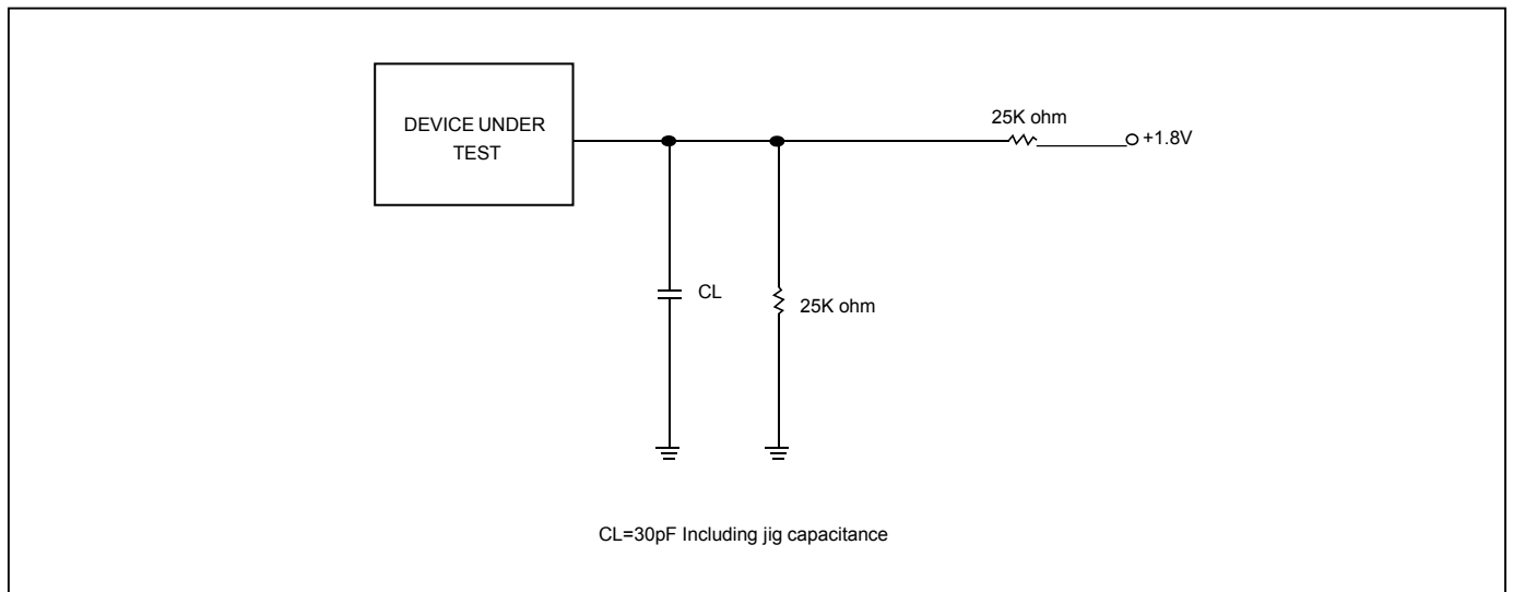
Figure 75. Output Loading
