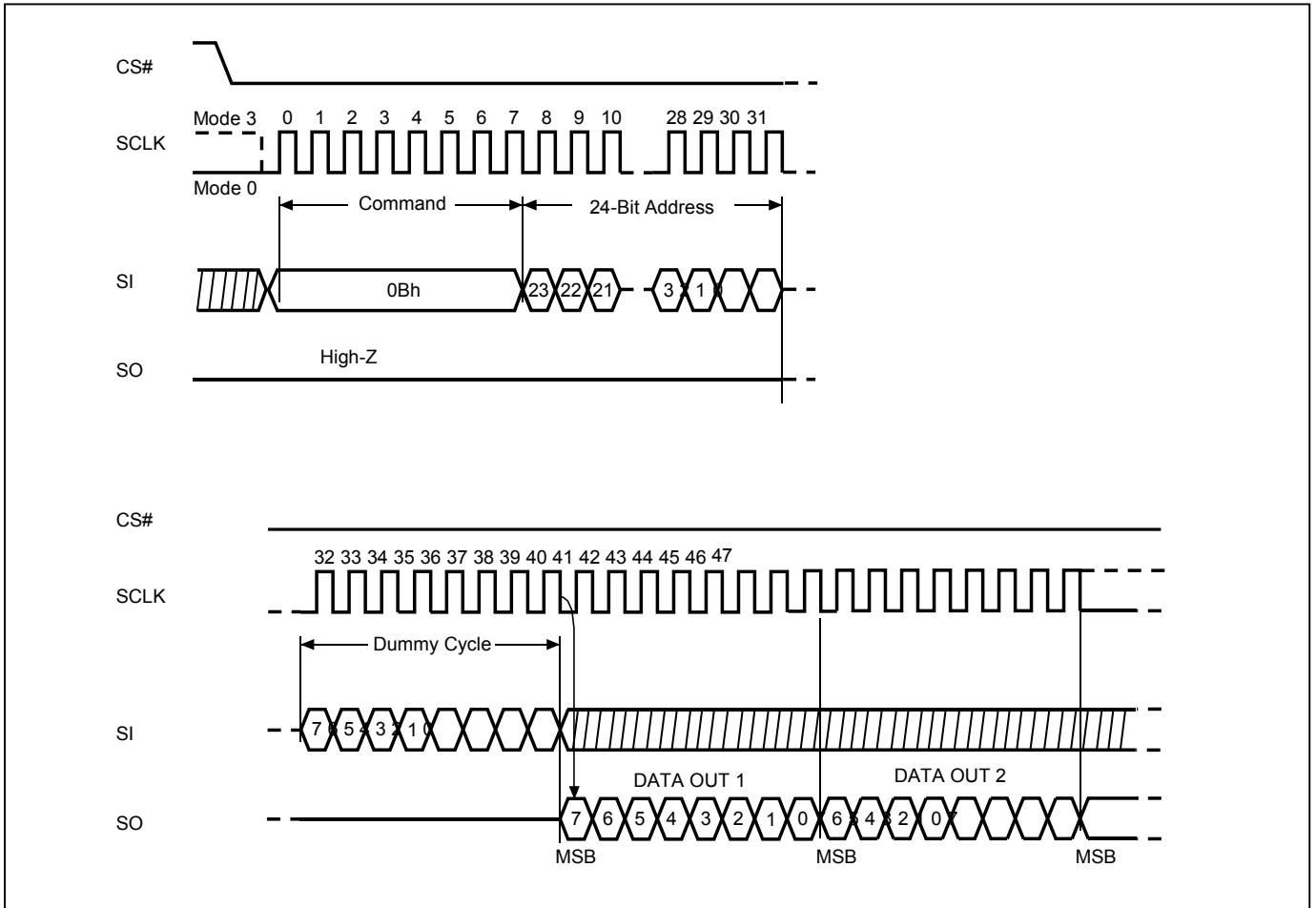
Figure 27. Read at Higher Speed (FAST_READ) Sequence (SPIMode)
