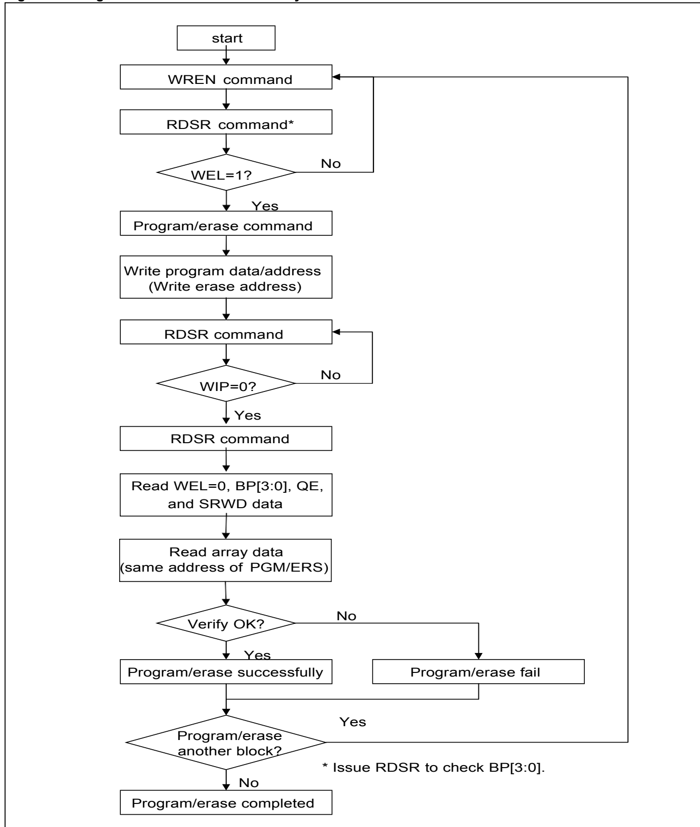
Figure 21. Program/Eraser flow with read array data
