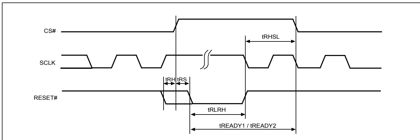
Figure 71. RESET Timing
