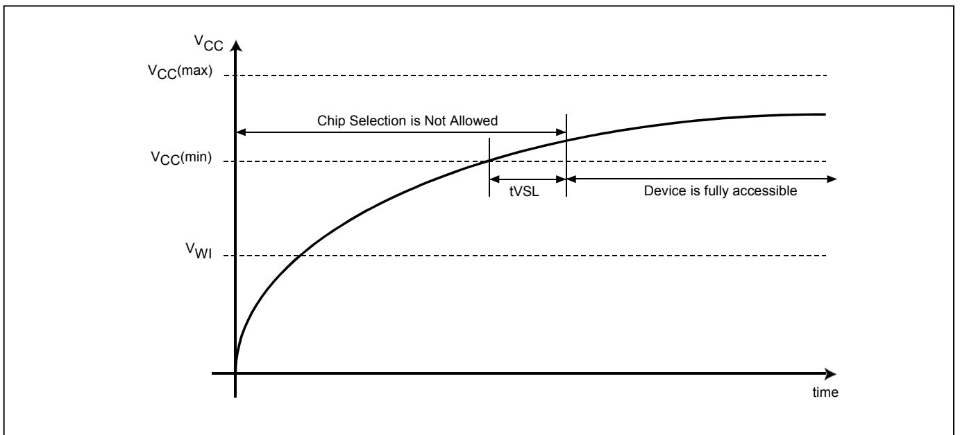
Figure 45. Power-up Timing
