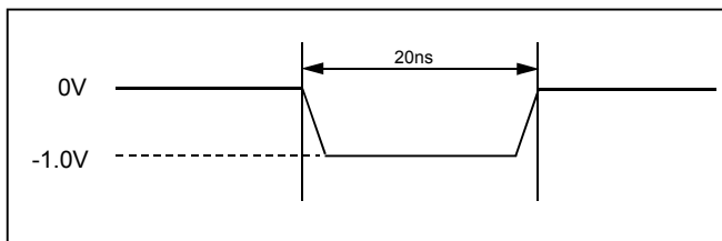
Figure 39. Maximum Negative Overshoot Waveform
