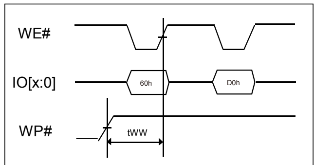
Figure 38-3. Enable Erasing of WP# Signal
