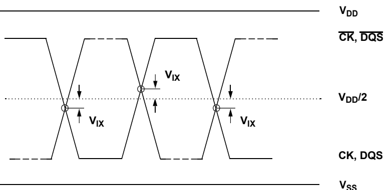
Figure 4. V_{IX} Definition
