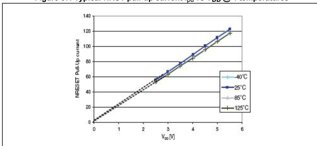
Figure 37. Typical NRST pull-up current I_{PU} vs V_{DD} @ 4 temperatures
