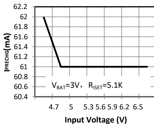
Pre-Charge Current vs. Input Voltage
