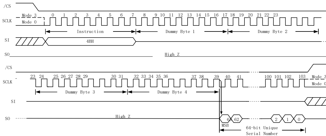
Figure 24. Read Unique ID Sequence Diagram (SPI Mode only)
