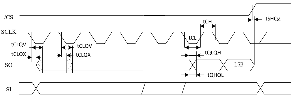
Figure 24. Output Timing
