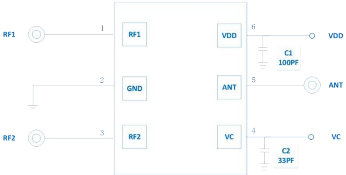
Figure 2 Application Schematic
