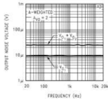
Noise Floor
